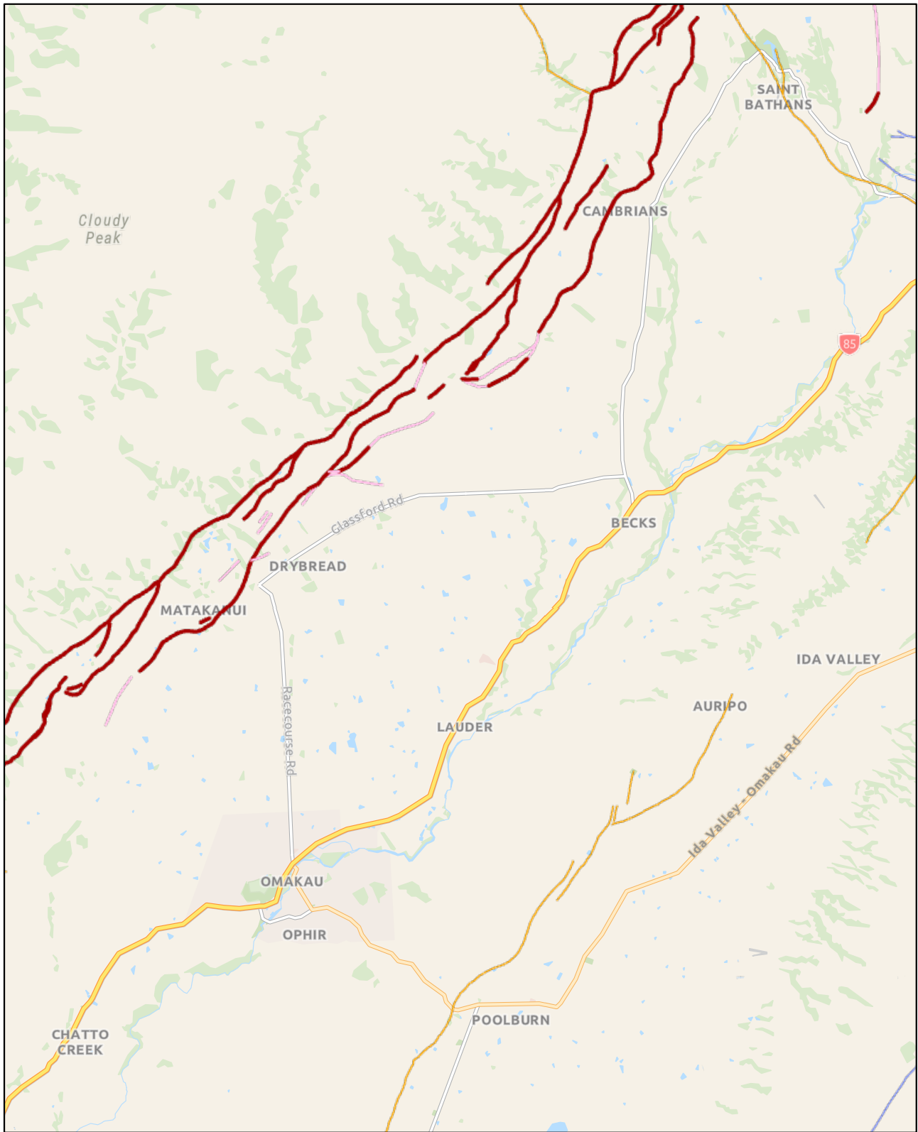
Manuherikia Valley - Active Fault Lines
